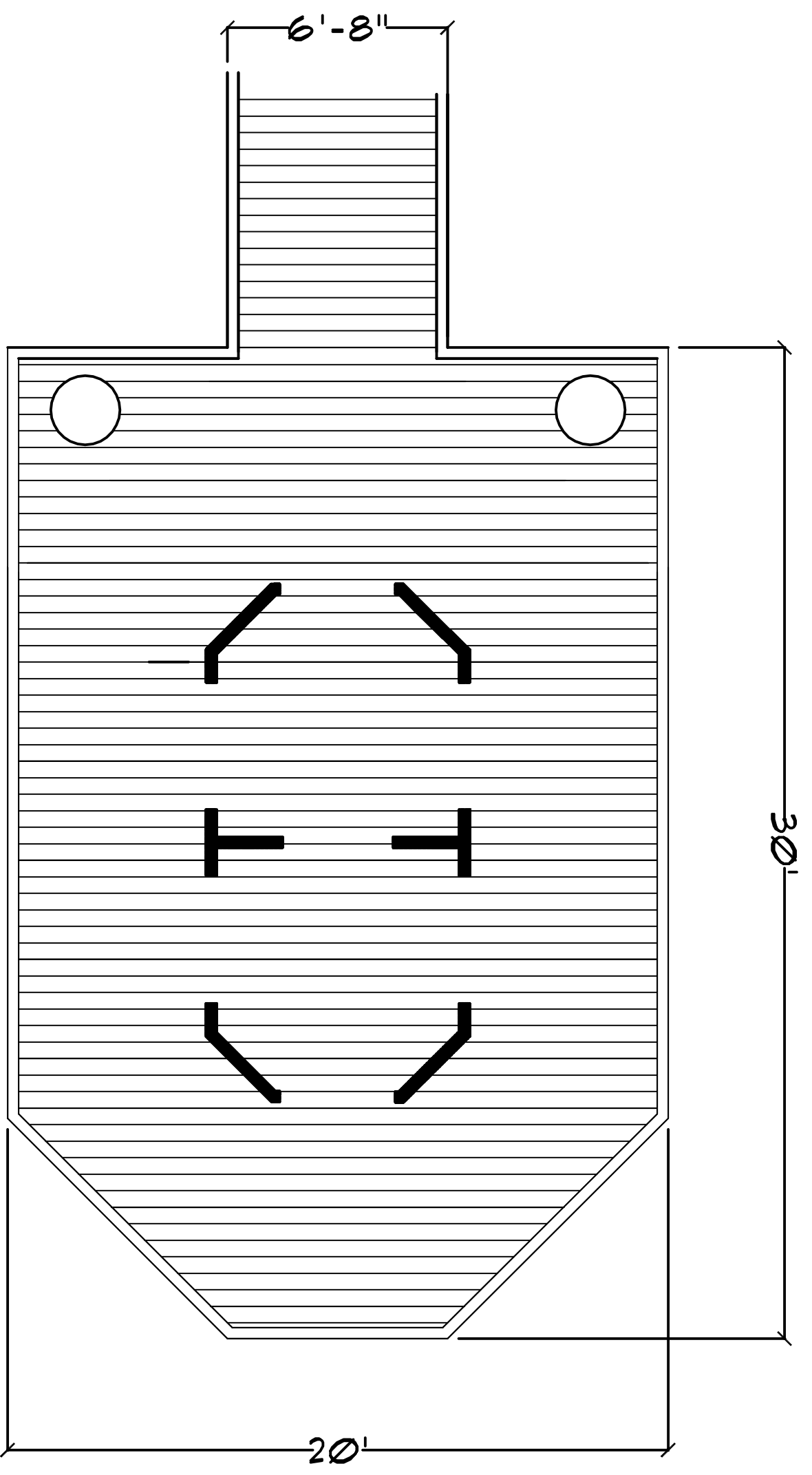
MAIN DECK PLAN SCALE: 1/4"
